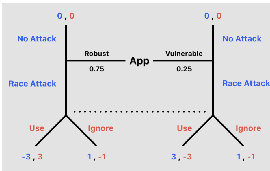
Figure 3: Game theory tree
