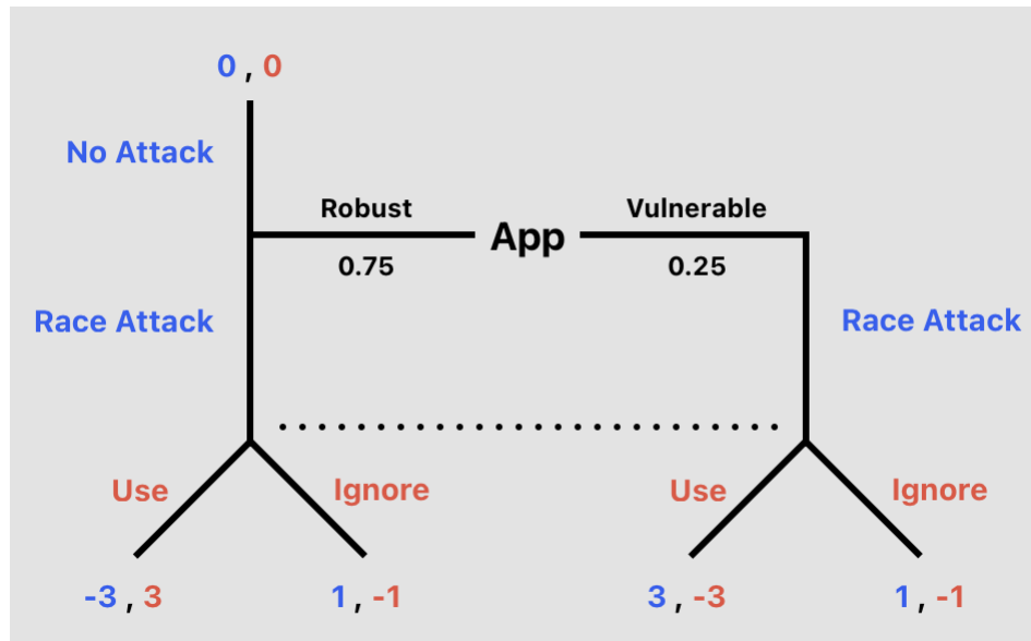
Figure 4: Player 1's profitable deviation
