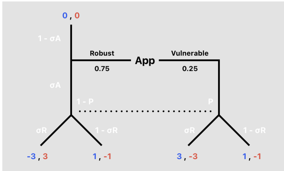
Figure 5: Mixed strategy tree
